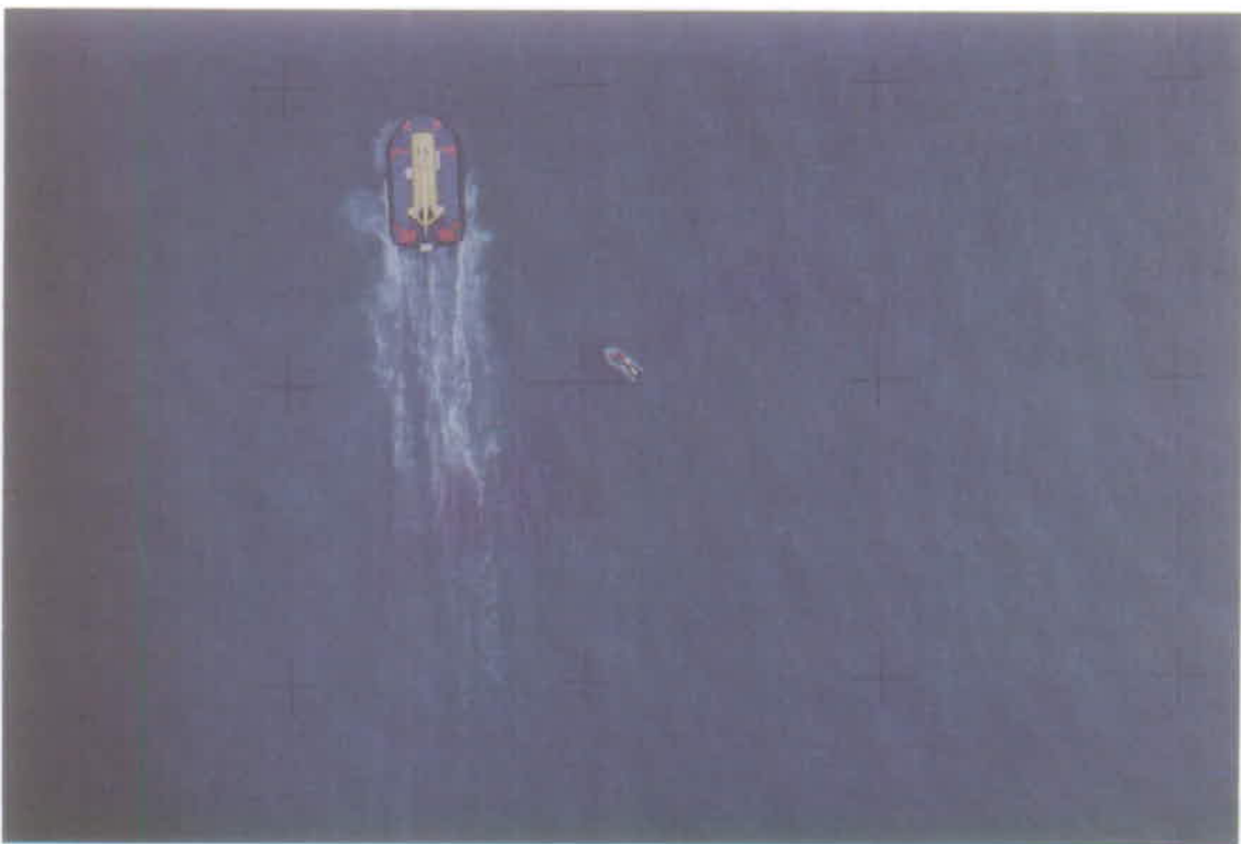
Figure 15. Two views showing the hovercraft proceeding at 21 knots through a dyed Canola oil slick (Run No. 5)
