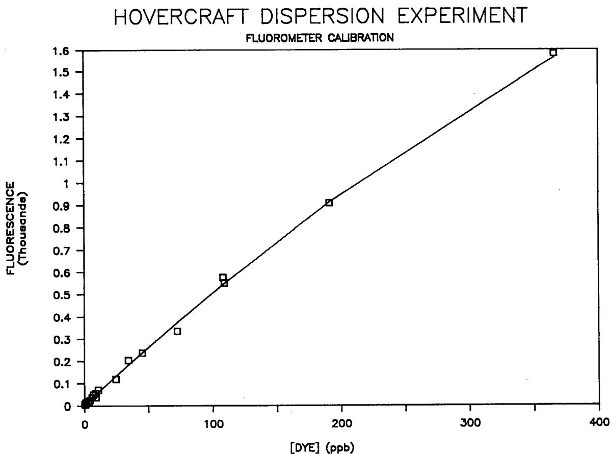
Figure 8. Fluorometer calibration curve
