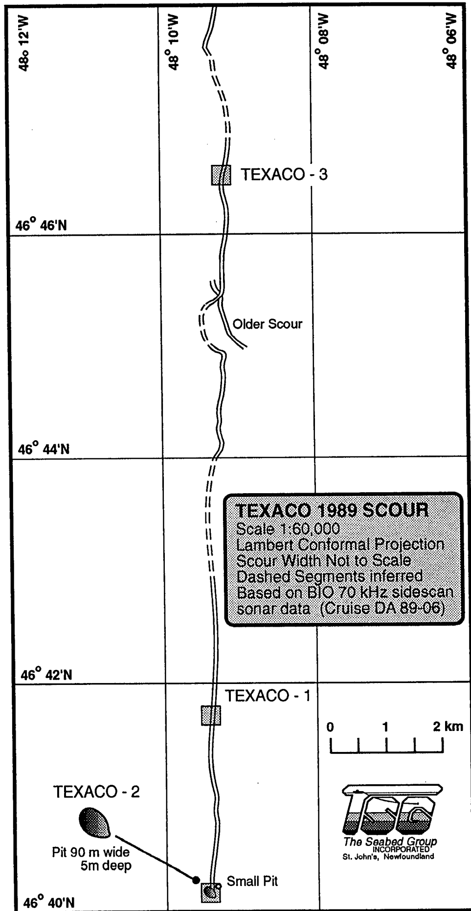
Figure 10. Reduced scale drawing of the Texaco 89-01 scour.
