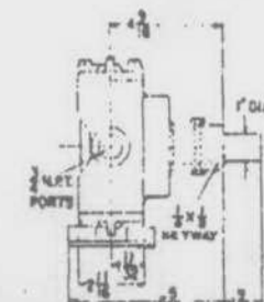
HOLLOW SHAFT MODELS with stub shaft No. 1300-5
