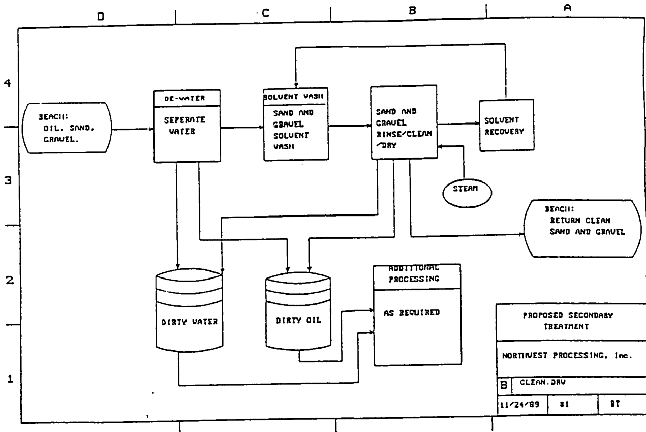
Figure 5: Proposed secondary treatment flowsheet for Northwest Processing System
