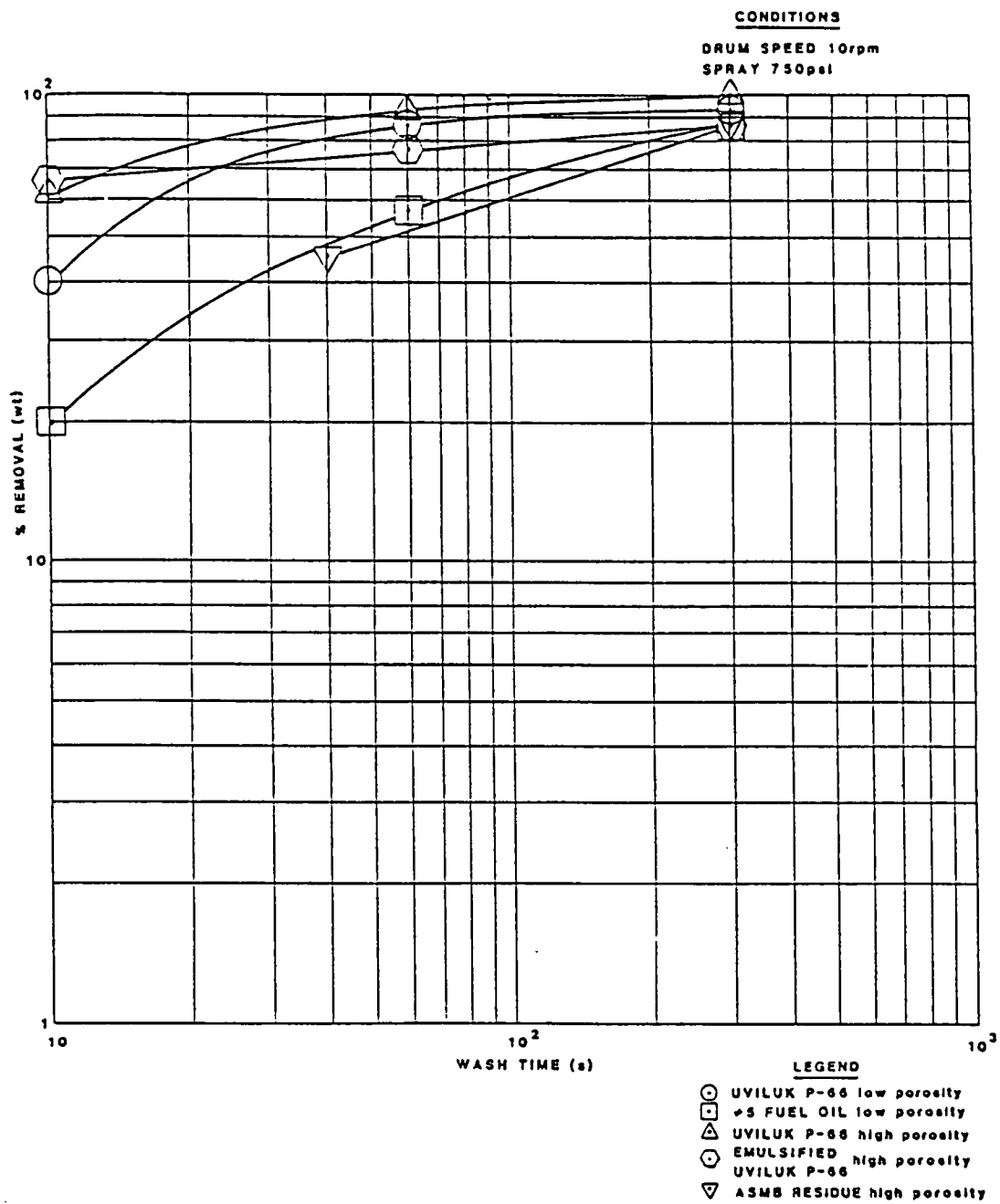
Figure 2: Percent removal vs. wash time
