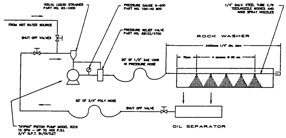
SPRAY HEADER PIPING SCHEMATIC
