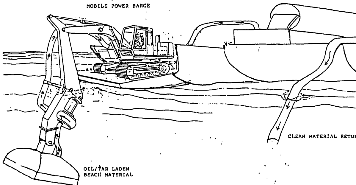
Figure 6: Northwest Processing beach cleaning system
