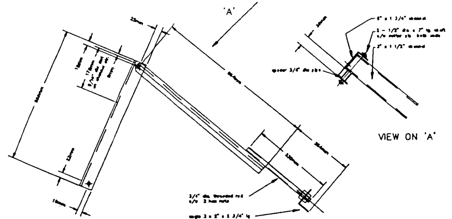
⑤ PULLEY SUPPORT 1 REQ'D
