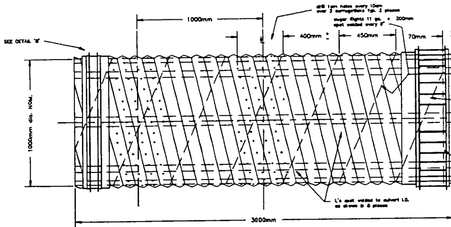
2 CORRUGATED CULVERT 1000mm dia. 1-REQ'D
