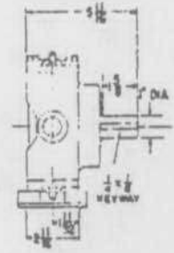
SOLID SHAFT MODELS
