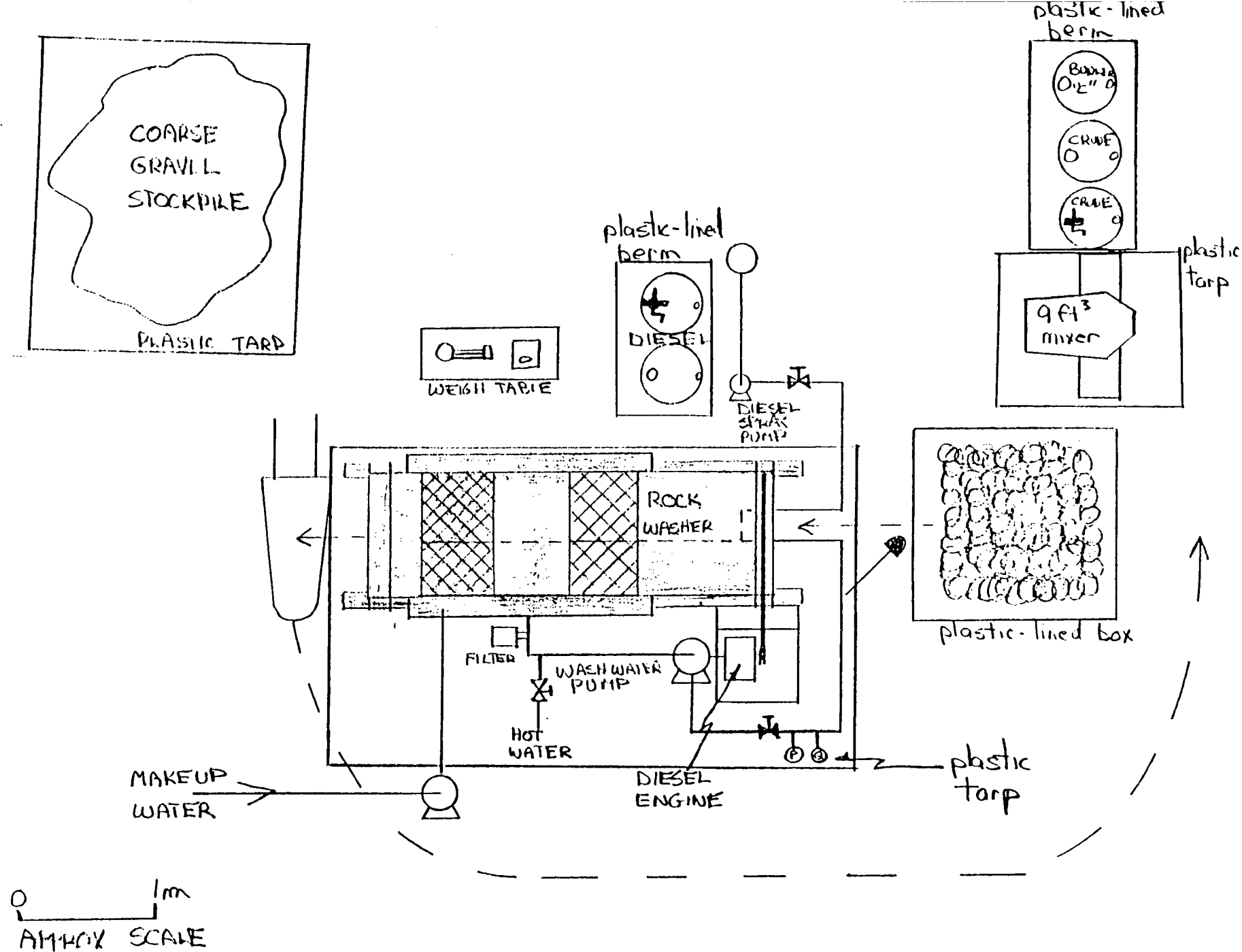
Figure 10: Test site layout
