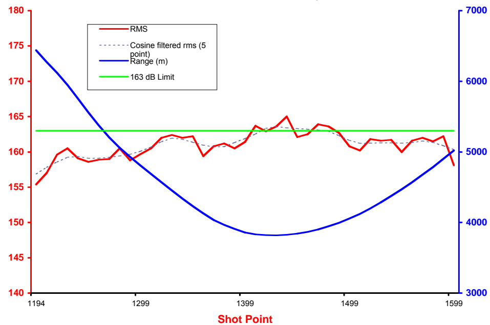
Acoustic Data - Northern Transect - 12 August 2001 4 km Line - 20 m Sonobuoy [T.4]
